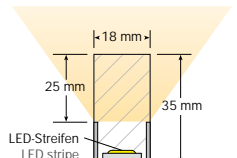
LED-Streifen LED stripe Bande LED Acryl Vollmaterial Acrylic solid material Entièrement en acrylique
